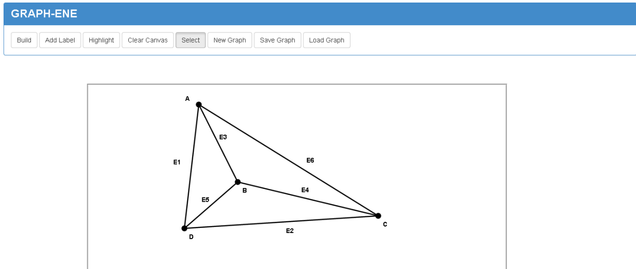
Figure 6 – Non-planar graph with crossing edges
