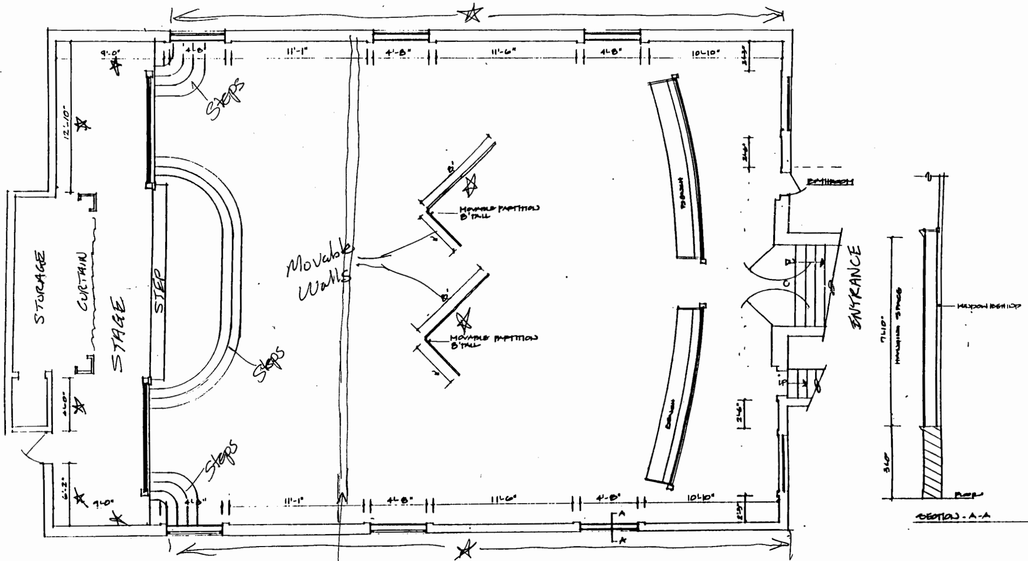
FLOOR PLAN - GALLERY X
